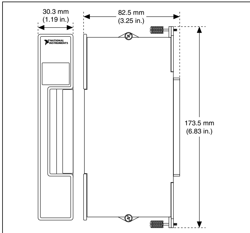
Figure 4. SCXI-1313A Dimensions
