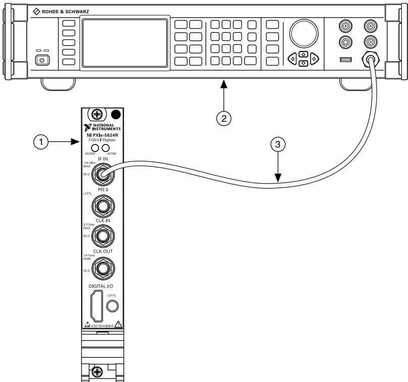
Figure 5. Internal Frequency Reference Adjustment Cabling Diagram
