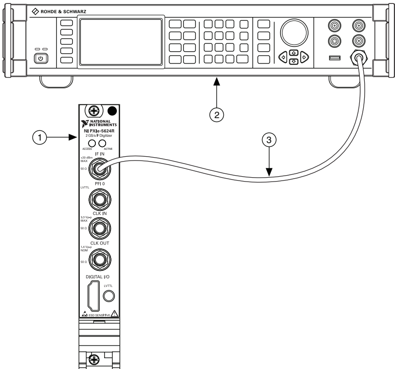
Figure 3. Internal Frequency Reference Verification Cabling Diagram
