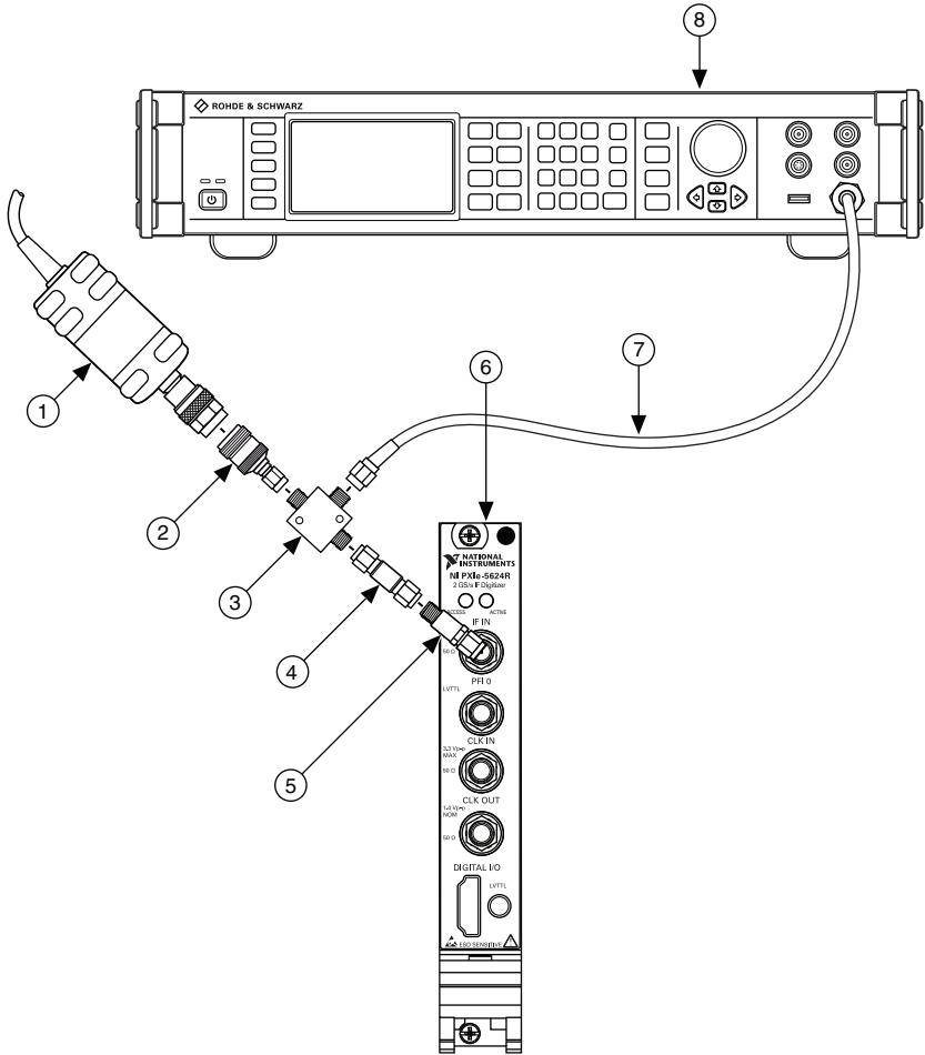
Figure 4. Absolute Amplitude Accuracy Verification Cabling Diagram
