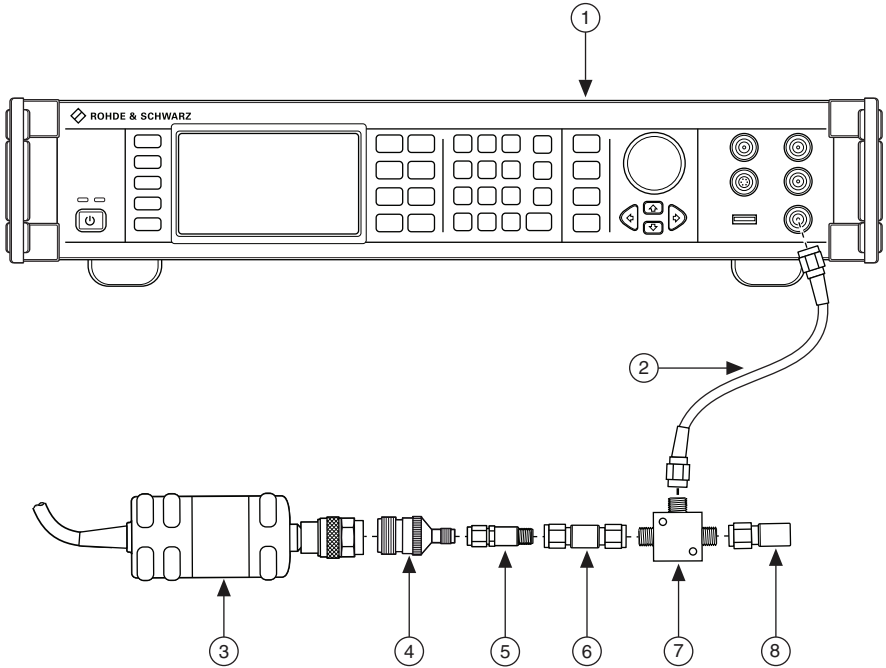
Figure 1. Connection Diagram for Measuring at Splitter Output 2
