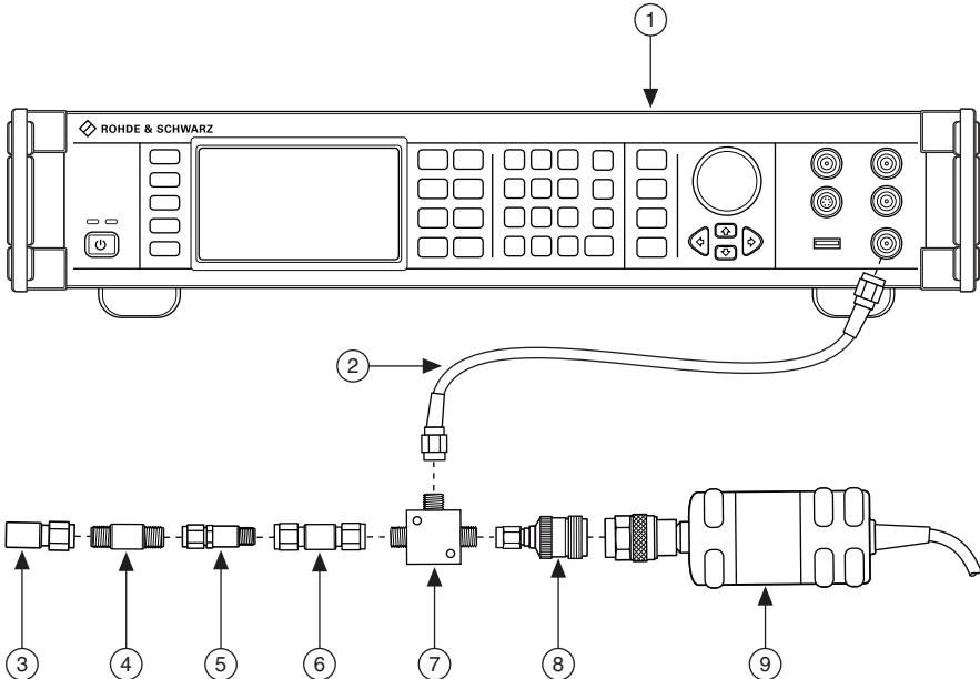
Figure 2. Connection Diagram for Measuring at Splitter Output 1
