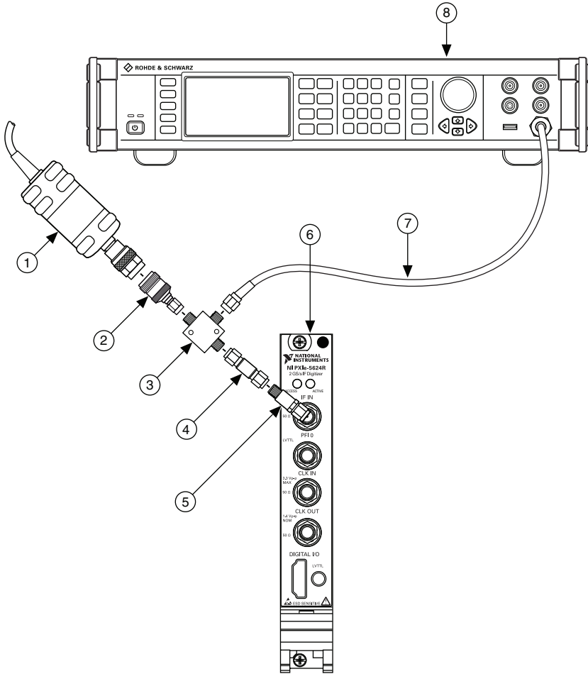
Figure 6. Absolute Amplitude Accuracy Adjustment Cabling Diagram
