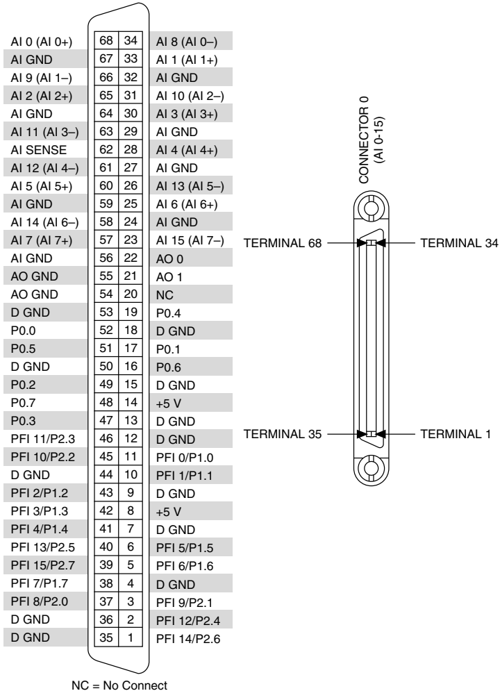
Figure 6. NI PCIe/PXIe-6341 Pinout
