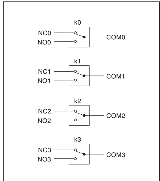
Figure 4. NI PXI-2548 Power-On State
