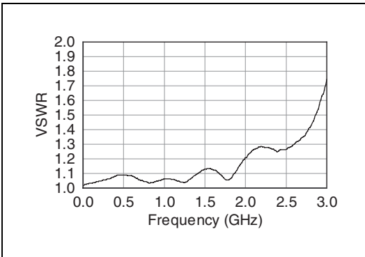
Figure 2. Typical VSWR
