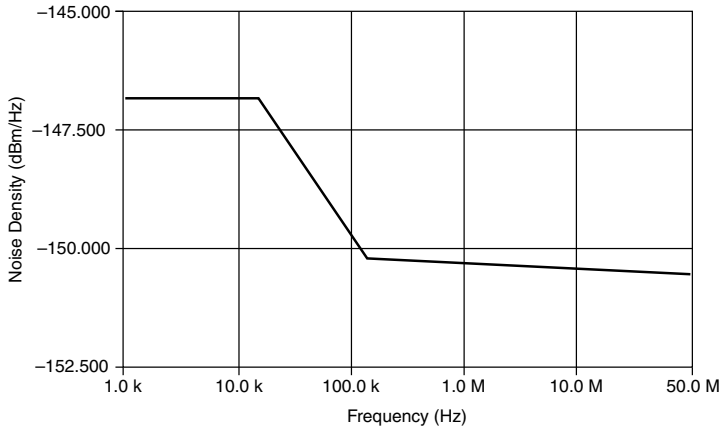
Figure 4. PCI-5142 Spectral Noise Density on 0.2 V Input Range, Noise Filter Enabled, 1 M \Omega Input Impedance, Nominal
