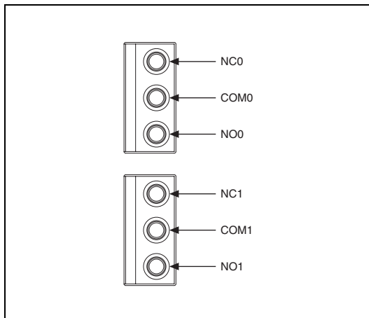
Figure 4. NI PXI-2599 Front Panel Connectors
