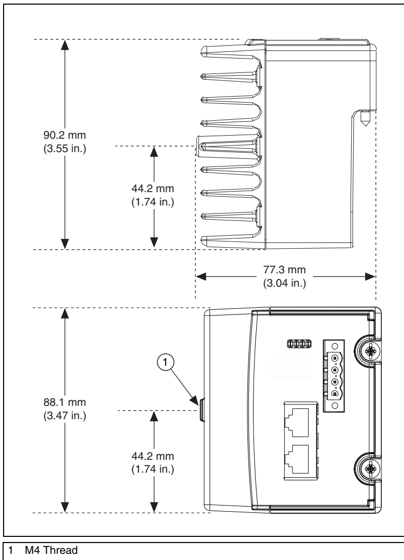
Figure 2. cRIO-9052 Front and Bottom Views with Dimensions
