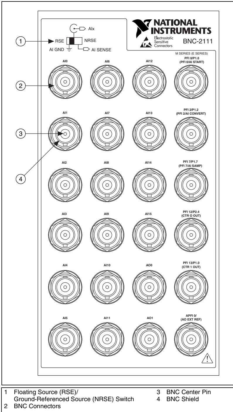
Figure 1. BNC-2111 Front Panel
