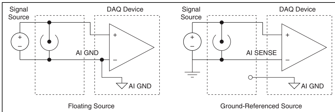
Figure 2. BNC-2111 Signal Source Types
