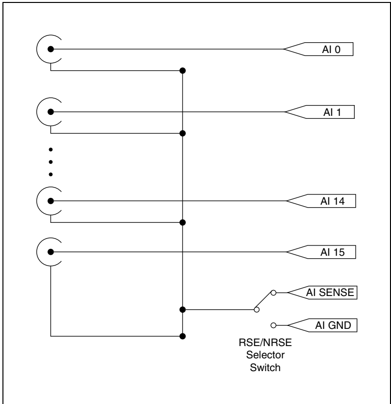
Figure 3. AI Channels 0–15 Connections
