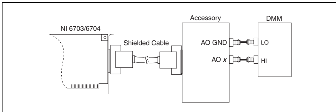
Figure 1. Calibration Connections
