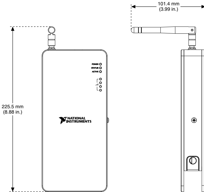
Figure 2. NI cDAQ-9191 Antenna Dimensions
