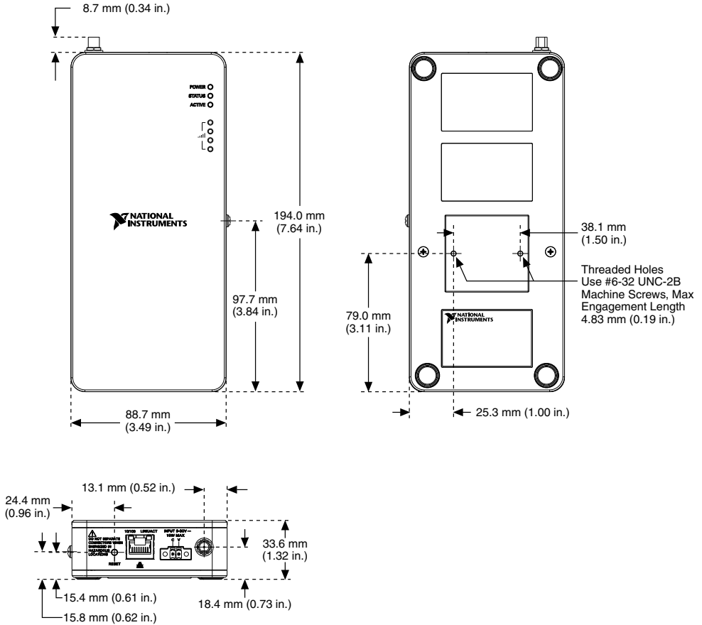
Figure 1. NI cDAQ-9191 Dimensions
