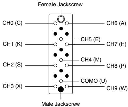
Figure 5. PXI-2585 Connector Pinout
