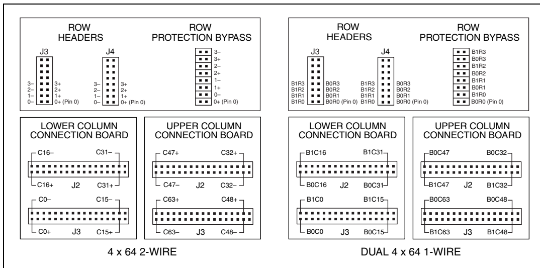
Figure 2. NI TB-2643 Terminal Block Signal Connections
