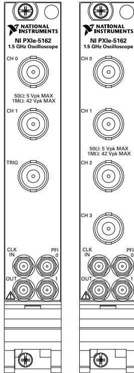
Figure 3. PXIe-5162 (2CH) and PXIe-5162 (4CH) Front Panels
