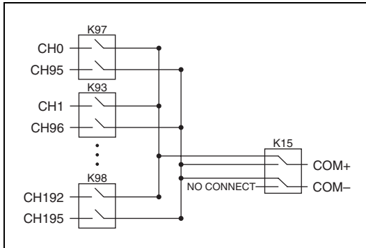
Figure 1. NI PXI-2575 Power-On State
