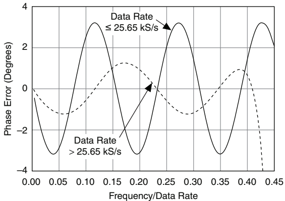
Figure 6. Phase Nonlinearity of the NI 9233
