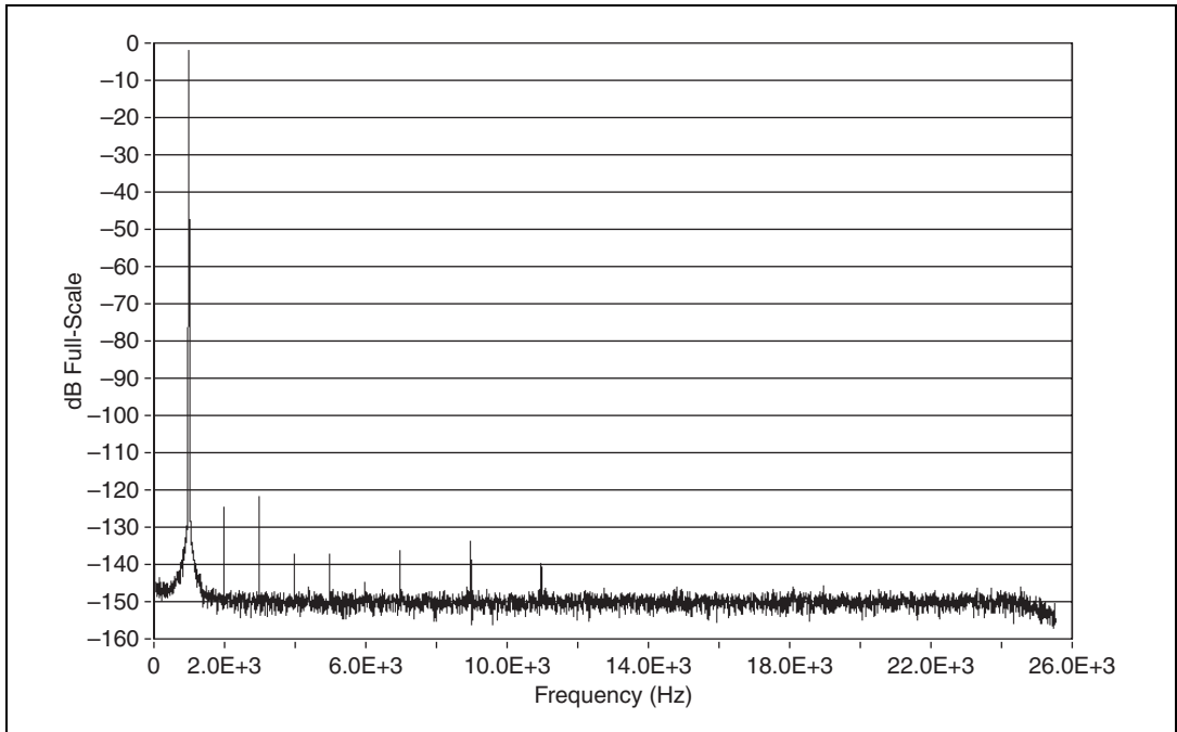
Figure 4. SFDR 51.2 kS/s (-1 dBFS, 0 dB Gain, 1 kHz Sine Wave Input)
