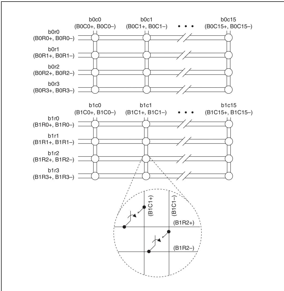
Figure 1. NI 2529 2-Wire Dual 4 x 16 Matrix Configuration
