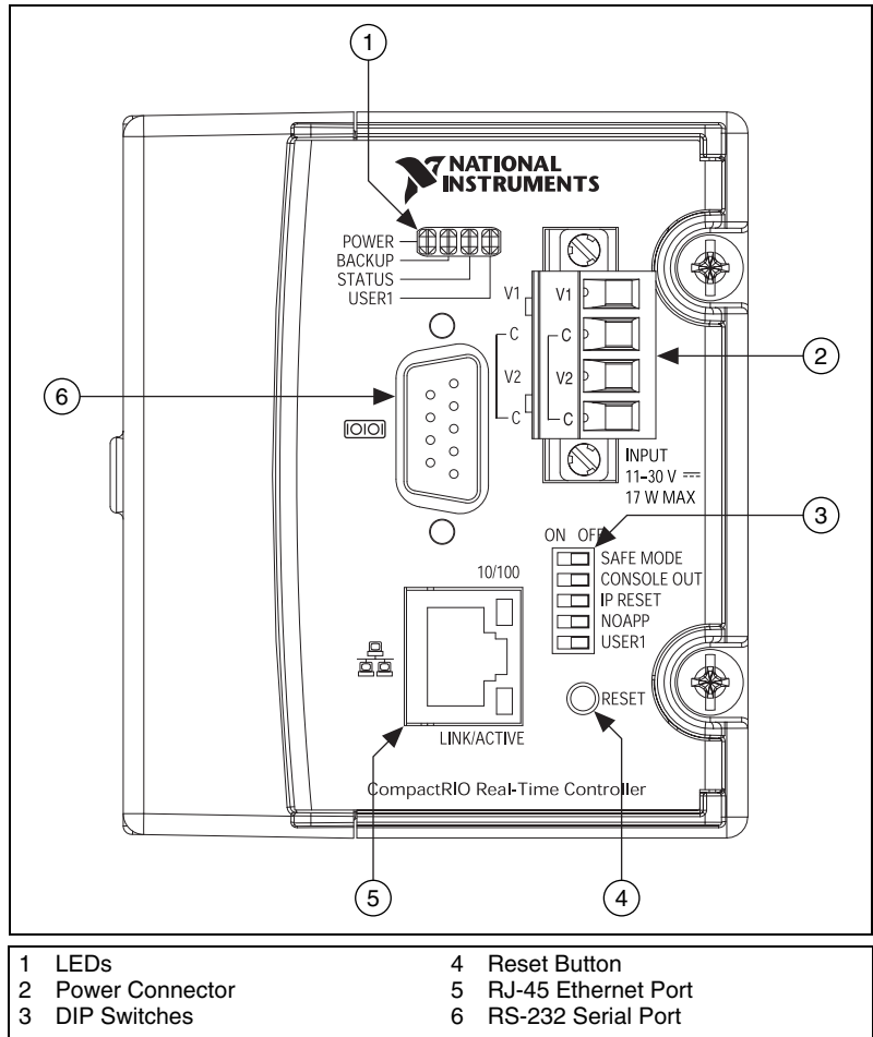
Figure 1. CompactRIO cRIO-9002/9004
