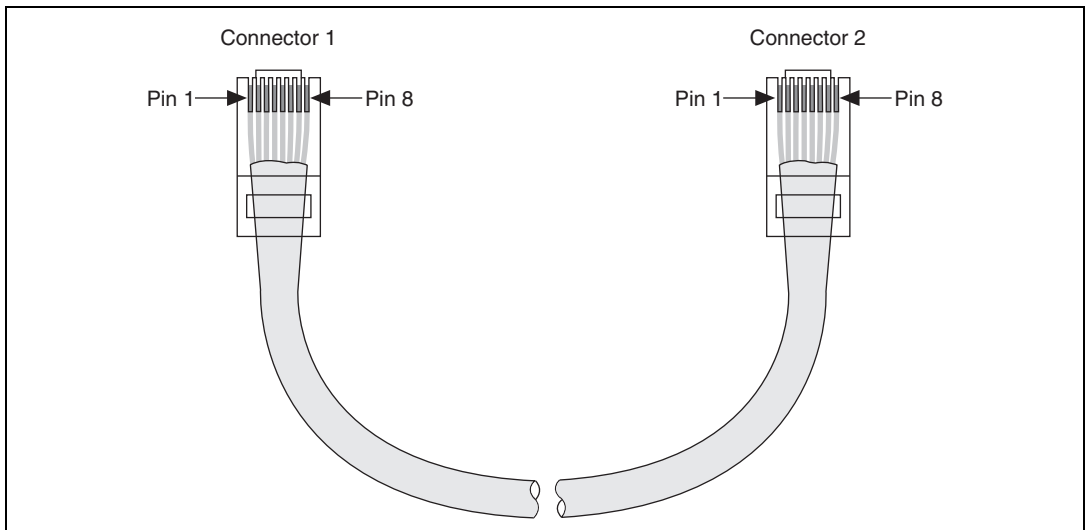
Figure 6. Ethernet Connector Pinout
