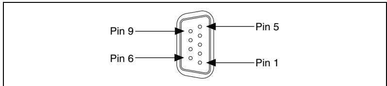
Figure 3. Controller Serial Port
