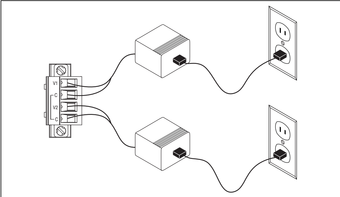
Figure 2. Wiring Power to the Controller
