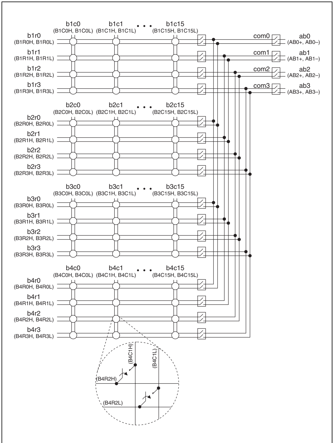
Figure 1. NI SCXI-1129 Quad 2-Wire 4 × 16 Matrix Topology
