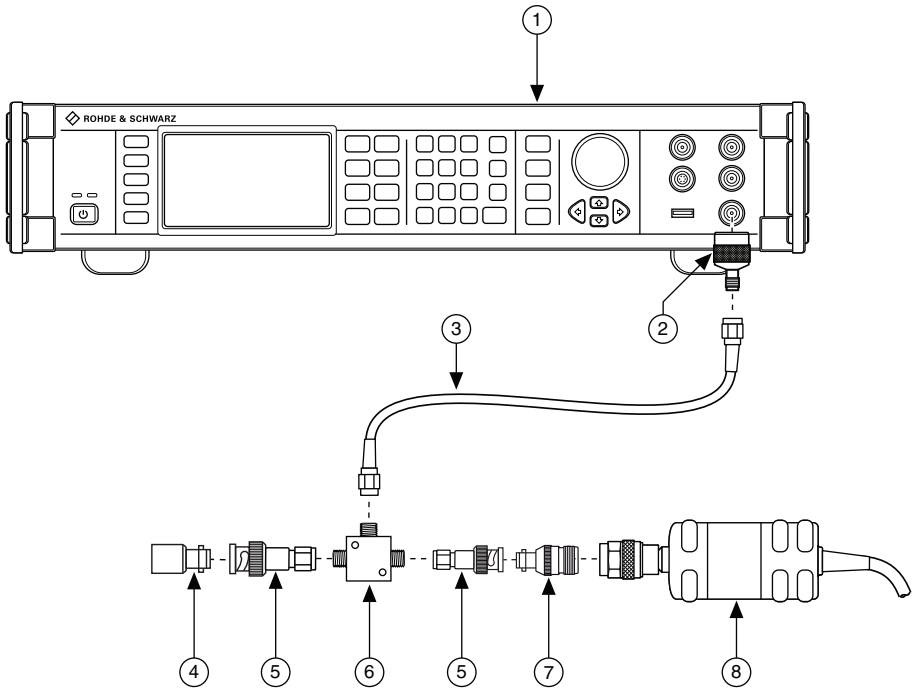
Figure 3. Connection Diagram for Measuring at Splitter Output 2 (BNC)
