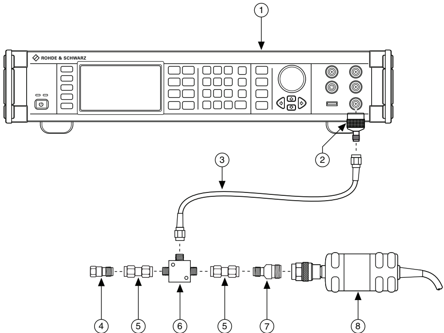
Figure 1. Connection Diagram for Measuring at Splitter Output 2 (SMA)
