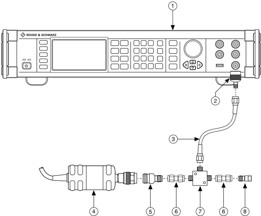
Figure 2. Connection Diagram for Measuring at Splitter Output 1 (SMA)
