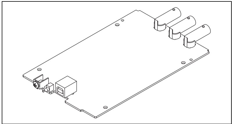
Figure 1. USB-5132/5133 OEM Device
