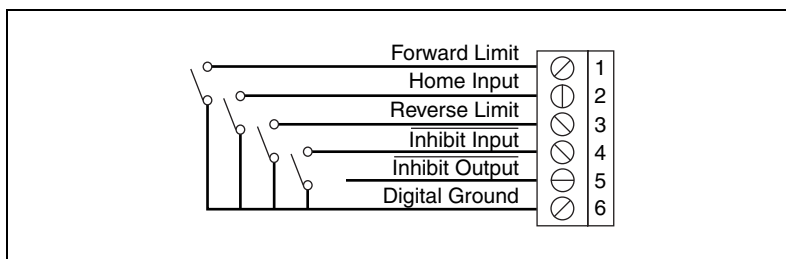
Figure 11. Limit Switch Terminal Block Pin Assignment (Passive Limit Switch Connection Example)
