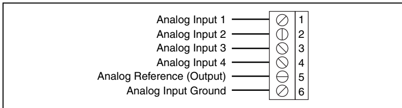
Figure 14. Analog Input Terminal Block Pin Assignment
