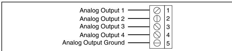
Figure 15. Analog Output Terminal Block Pin Assignment
