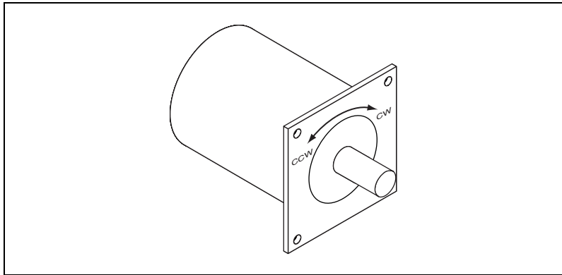
Figure 9. Clockwise and Counter-Clockwise Motor Rotation
