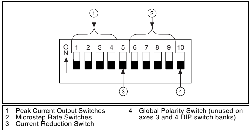
Figure 4. DIP Switch Bank Layout
