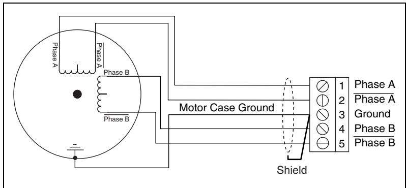
Figure 22. 4-Wire Motor Wiring
