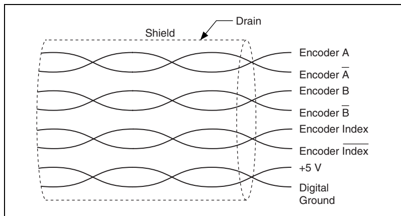
Figure 10. Shielded Twisted Pairs
