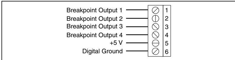
Figure 13. Breakpoint Terminal Block Pin Assignment
