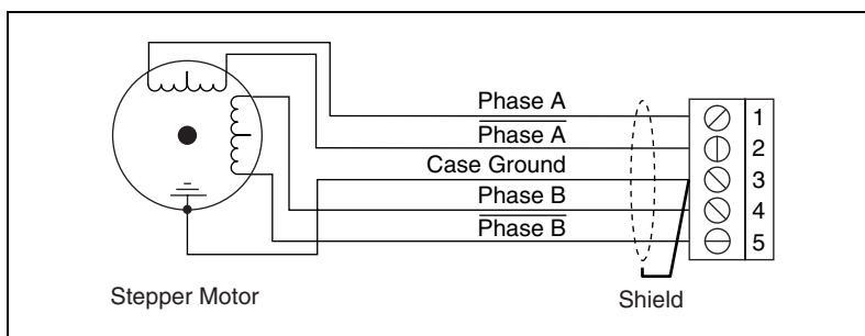
Figure 5. Typical Full-Coil Stepper Motor (2-Phase Type) Terminal Block Pin Assignment
