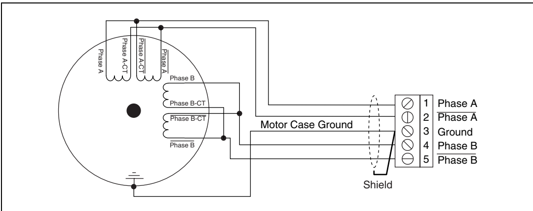
Figure 20. Parallel Stepper Motor Wiring (Higher Speed, Lower Torque)
