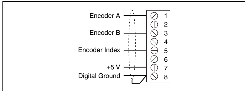
Figure 6. Typical Single-Ended Encoder Wiring Pin Assignment
