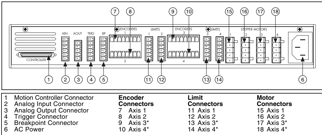
Figure 3. MID-7604/7602 Back Panel Connectors
