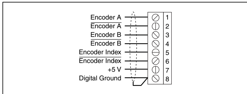
Figure 7. Typical Differential Line Driver Encoder Wiring Pin Assignment
