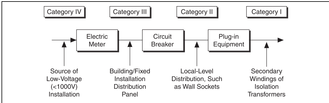
Figure 1. Sample Installation of the MID-7604/7602
