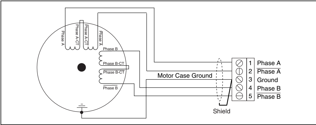
Figure 19. Series Stepper Motor Wiring (Higher Torque, Lower Speed)
