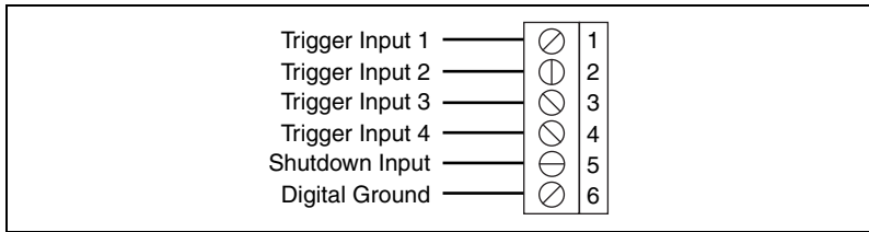
Figure 12. Trigger Terminal Block Pin Assignment
