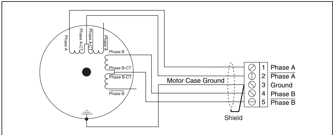
Figure 21. Half-Coil Stepper Motor Wiring
