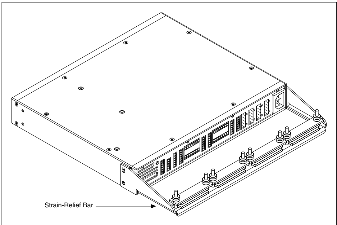
Figure 16. MID-7604/7602 with the Strain-Relief Bar Installed
