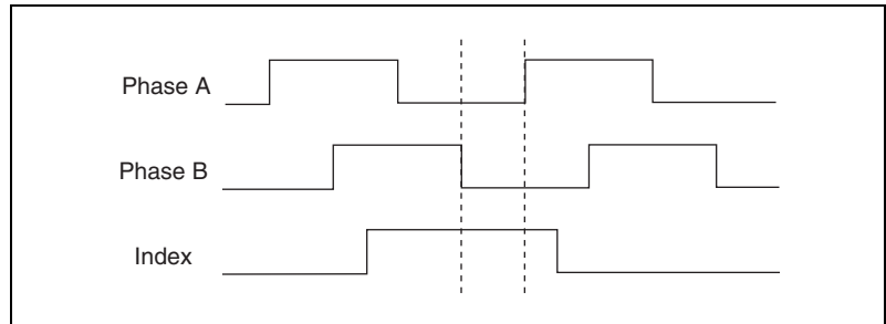
Figure 8. Encoder Signal Phasing, CW Rotation
