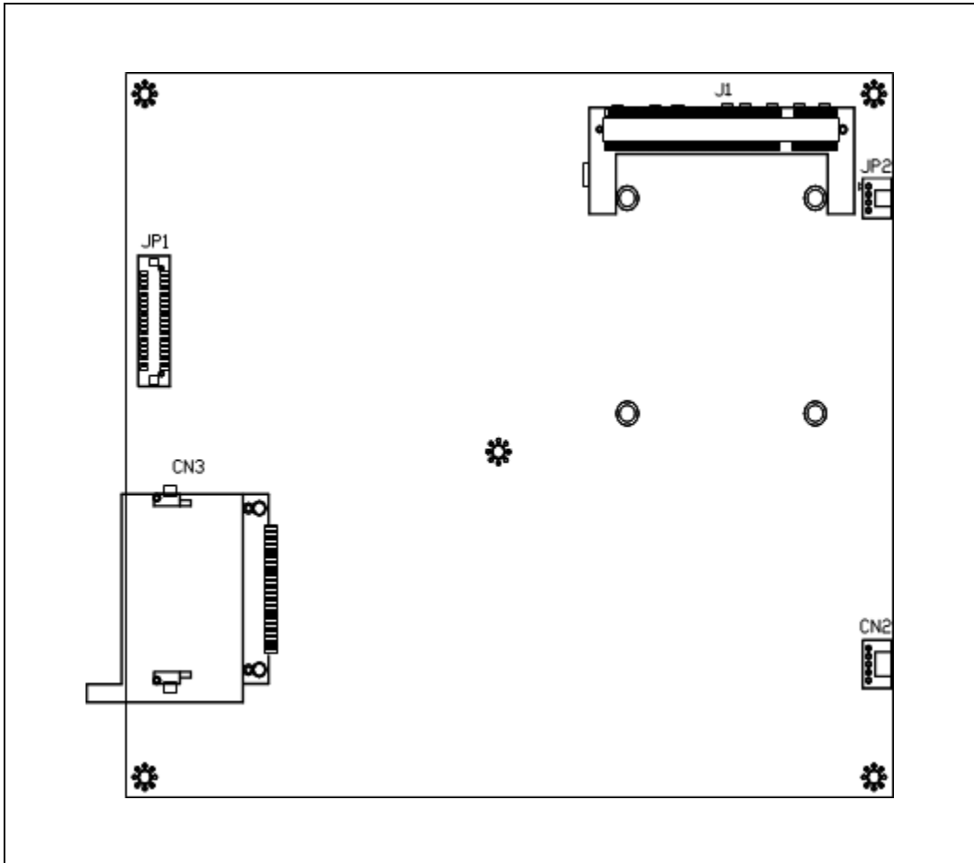
Figure 3-2. Main Board Jumpers and Connectors
