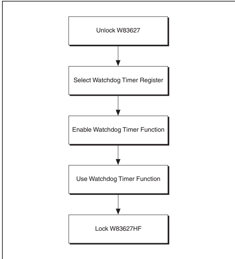
Figure C-1. Watchdog Timer Programming Procedure
