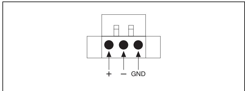
Figure 2-1. Power Connector
