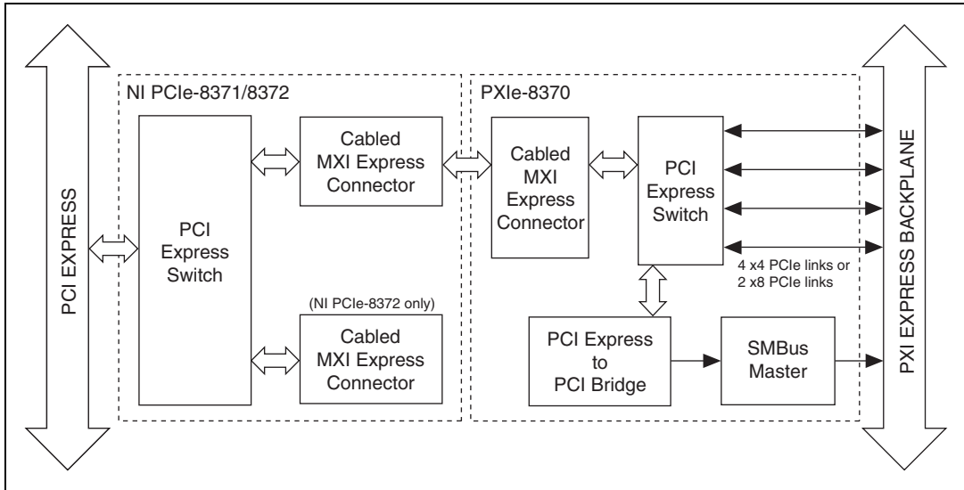
Figure 3-1. MXI-Express x4 Block Diagram
