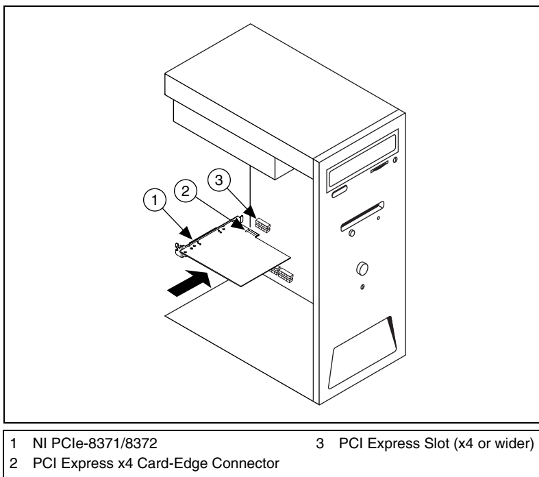
Figure 2-1. Installing the NI PCIe-8371/8372
