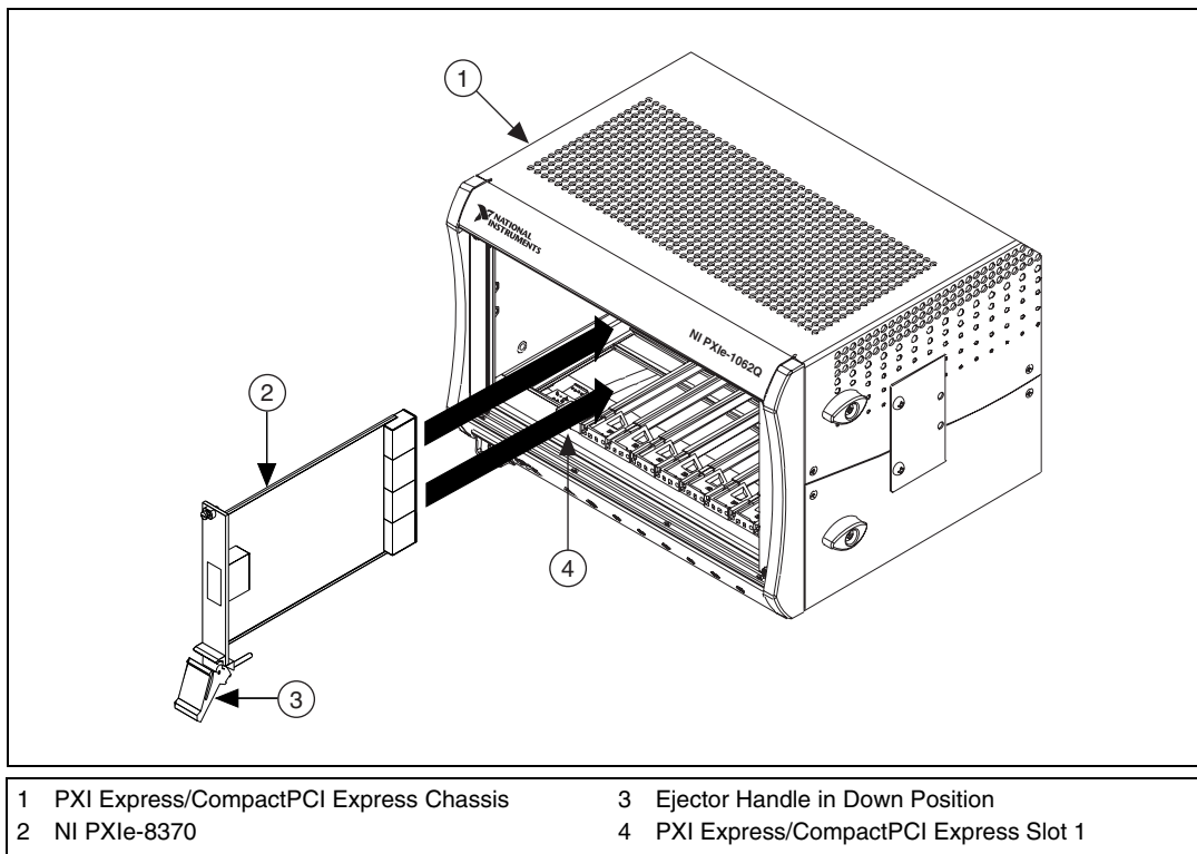
Figure 2-2. NI PXIe-8370 Card Before Installation
