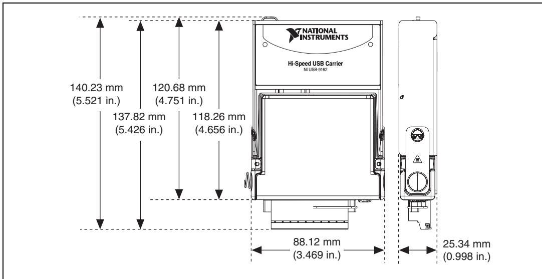
Figure 2. NI USB-9481 Device in Millimeters (Inches)
