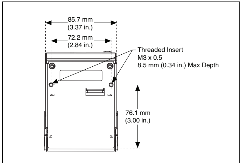
Figure 5. Module Dimensions In Millimeters (Inches)
