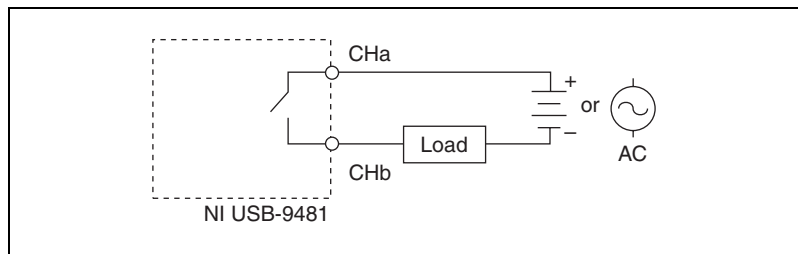
Figure 6. Connecting a Load to the NI USB-9481
