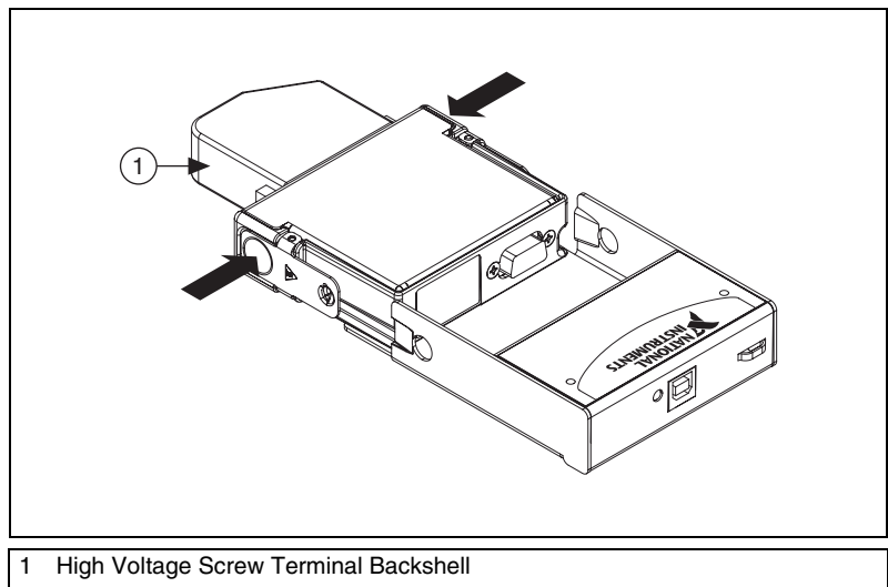
Figure 3. Module Installation
