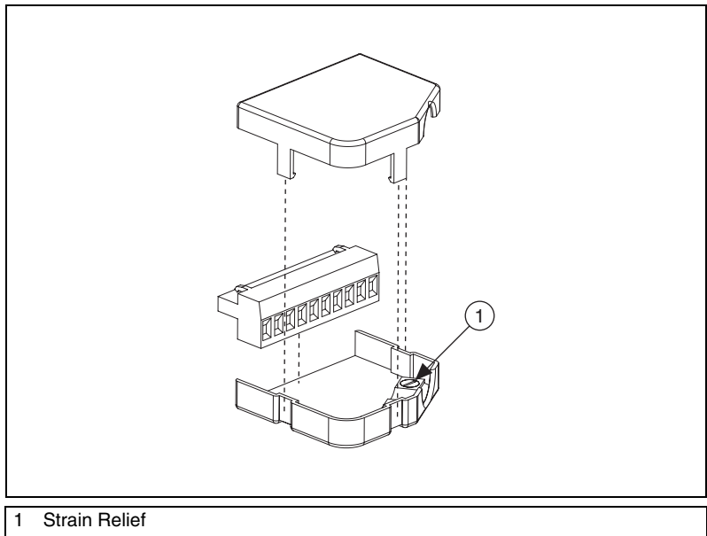
Figure 7. High Voltage Screw Terminal Backshell
