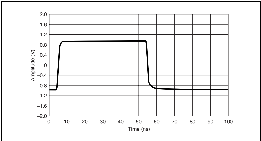
Figure 4. Pulse Response, Low-Gain Amplifier Path with a 50 Ω Load
