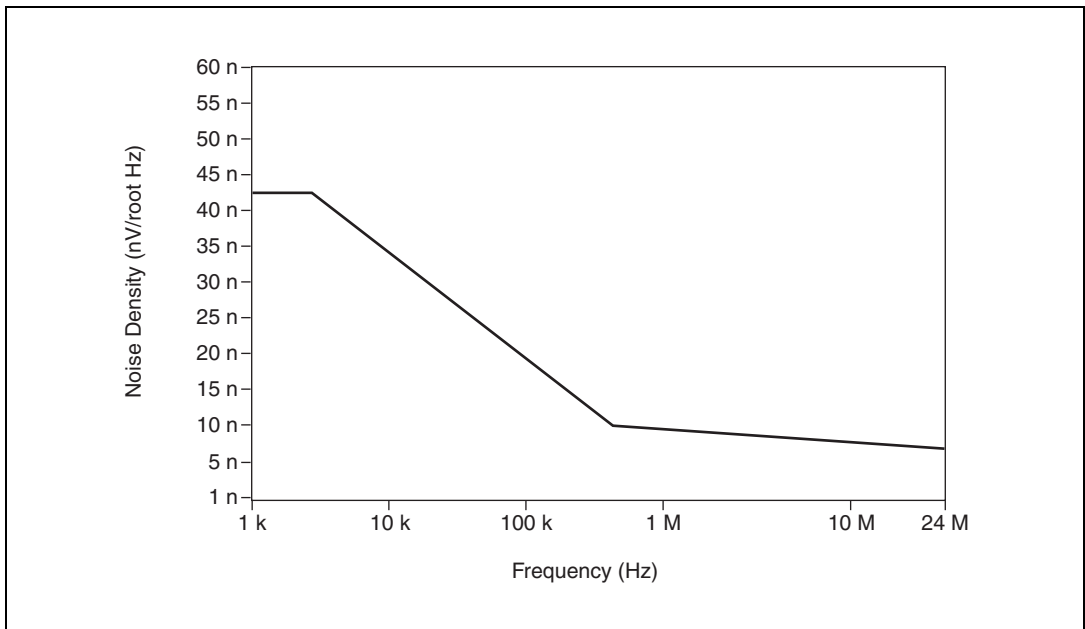
Figure 3. Representation of NI 5122 Spectral Noise Density on 0.2 V Range, Noise Filter Enabled, 1 M \Omega Input Impedance
