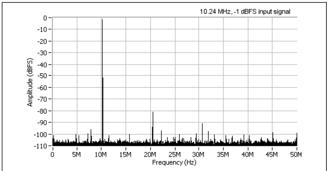
Figure 2. NI 5122 Dynamic Performance, 50 \Omega , 1 V_{pk-pk} Range (Typical)
