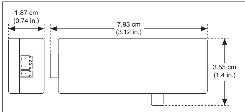
Figure 6. SCC-CO20 Dimensions
