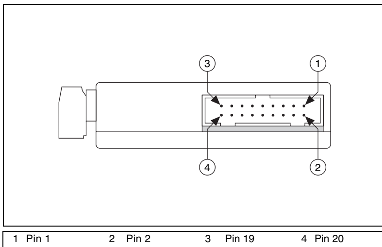
Figure 5. SCC Module Bottom View
