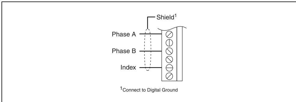
Figure 8. Single-Ended Encoder Pin Assignments
