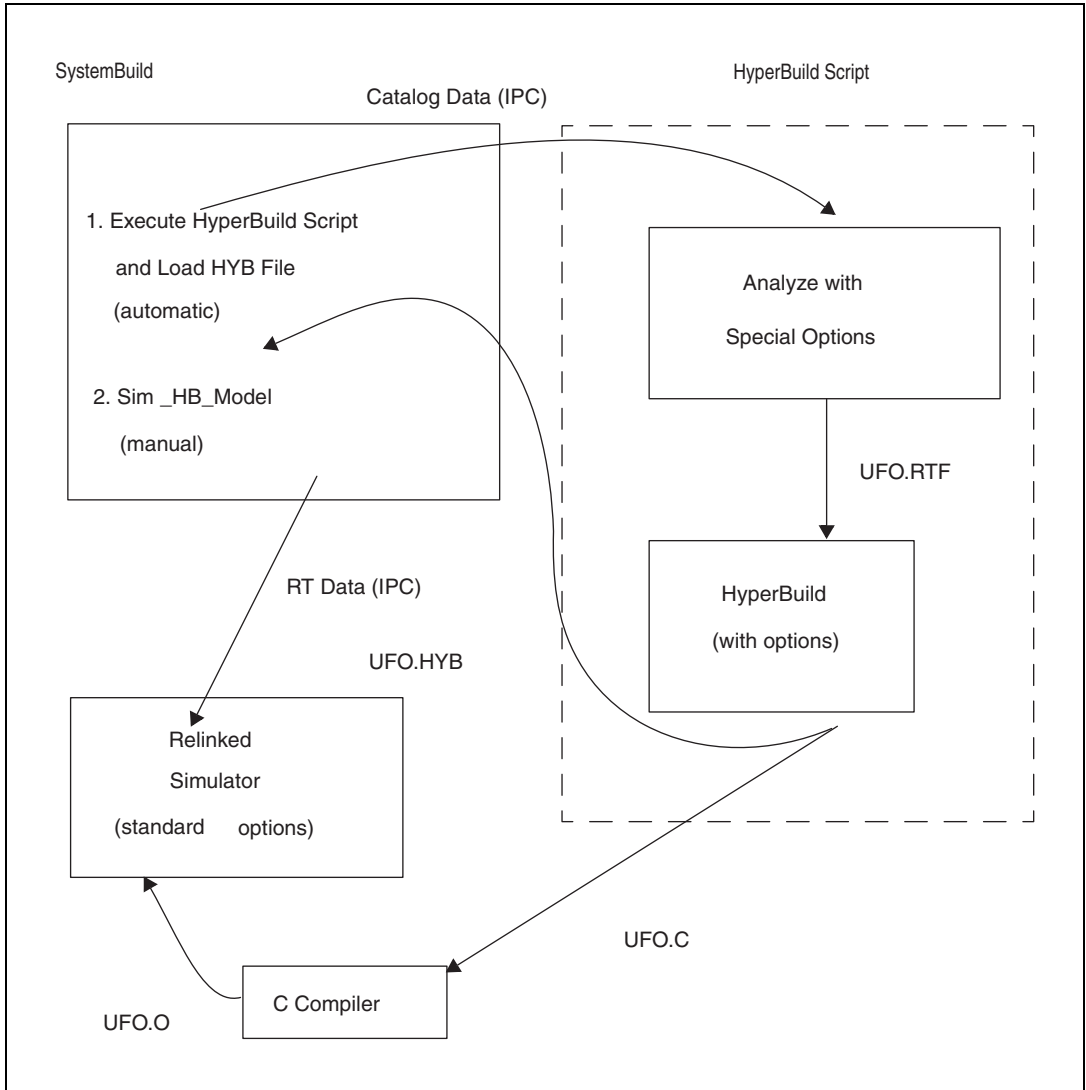
Figure 1-1. HyperBuild Simulation Process
