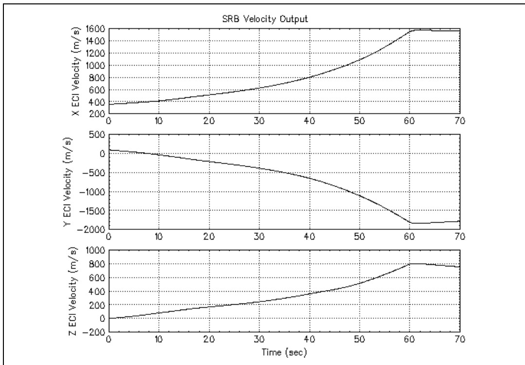
Figure 3-3. Velocity Output
