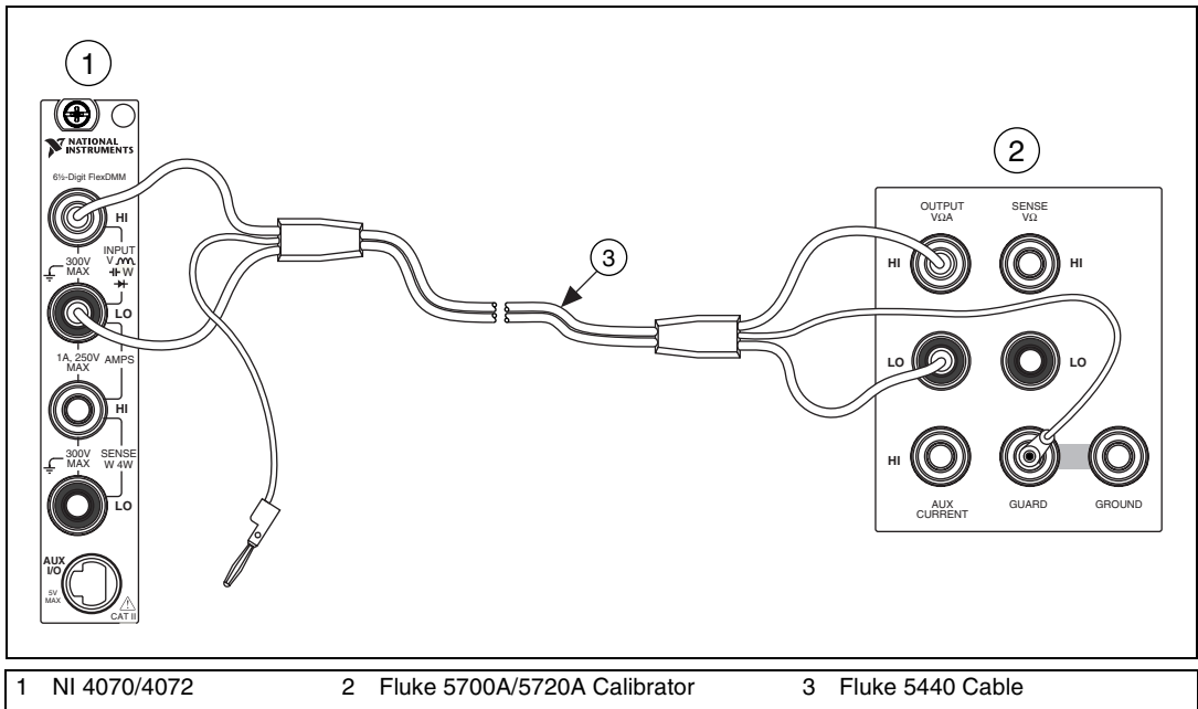
Figure 3. Cable Connections for Voltage and 2-Wire Resistance
