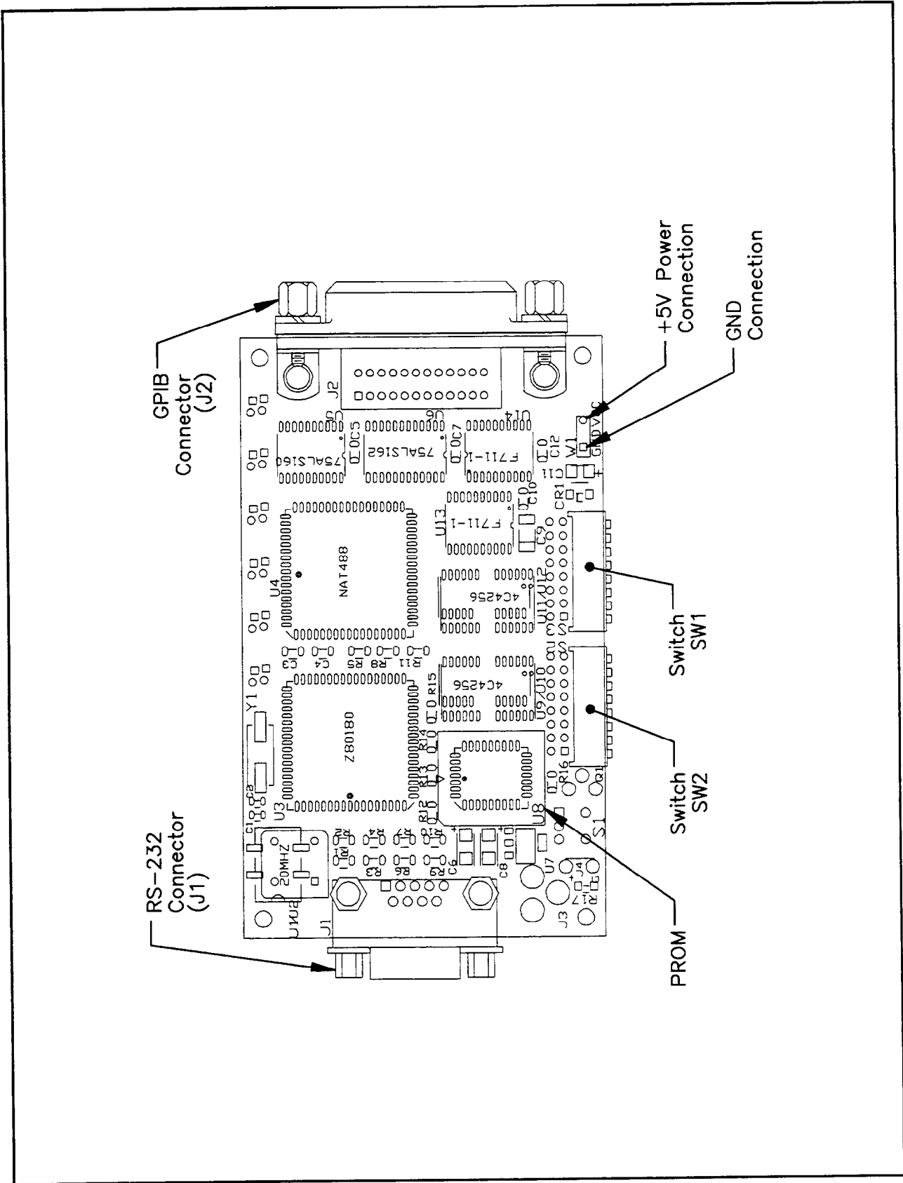
Figure 2. Component on the Bottom Side of the Circuit Card Assembly
