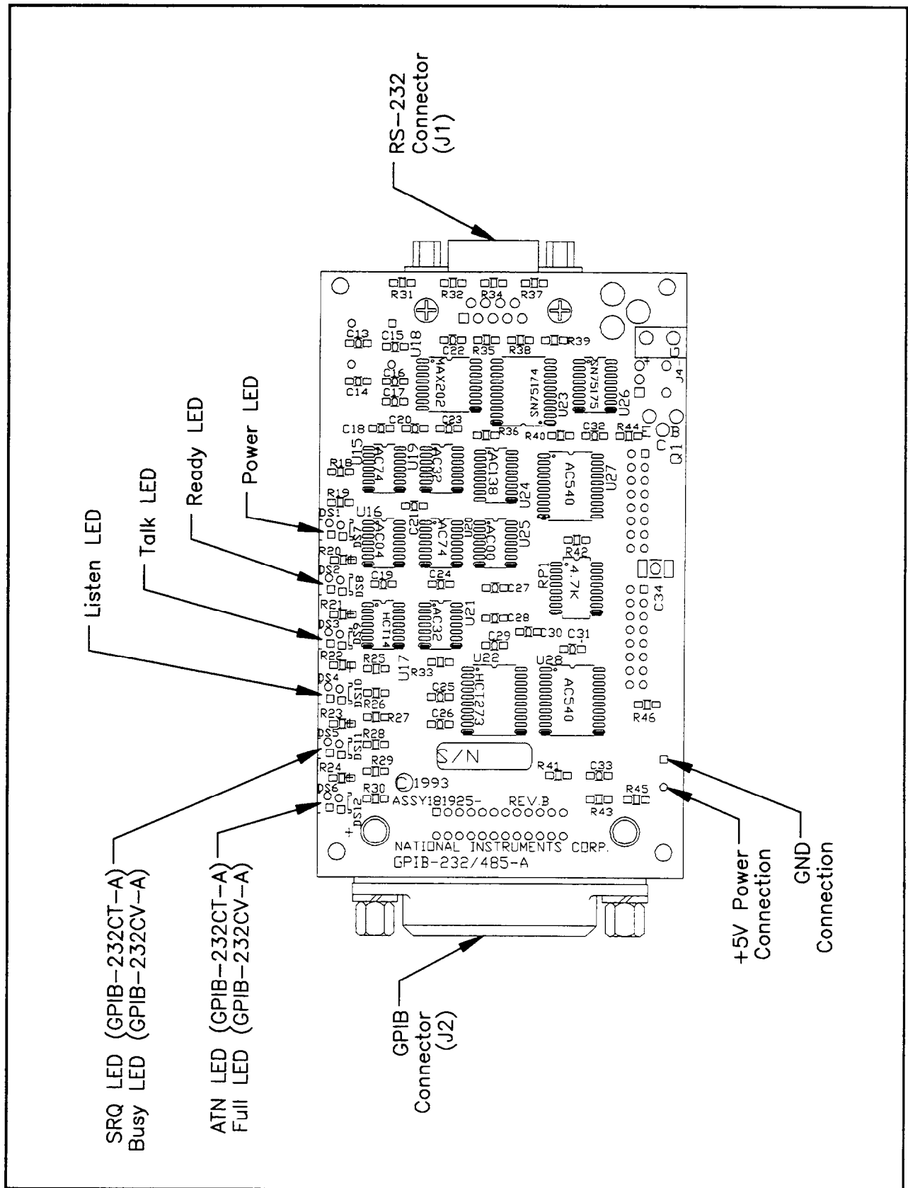
Figure 1. Component on the Top Side of the Circuit Card Assembly
