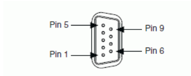
Controller Serial Port
