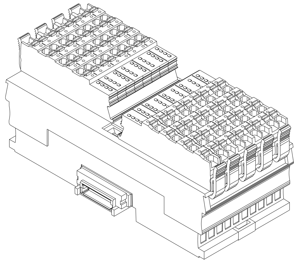
ISOMETRIC VIEW
